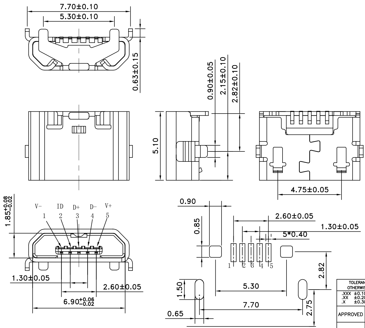
PCB LAYOUT
